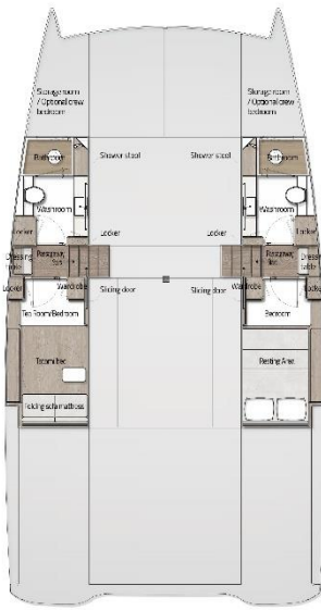
Interior Layout
